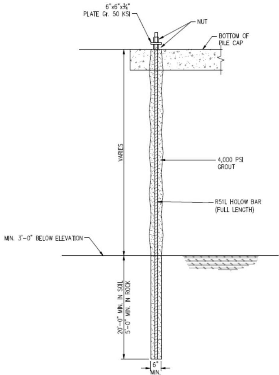
MICROPILE DETAIL NO SCALE
