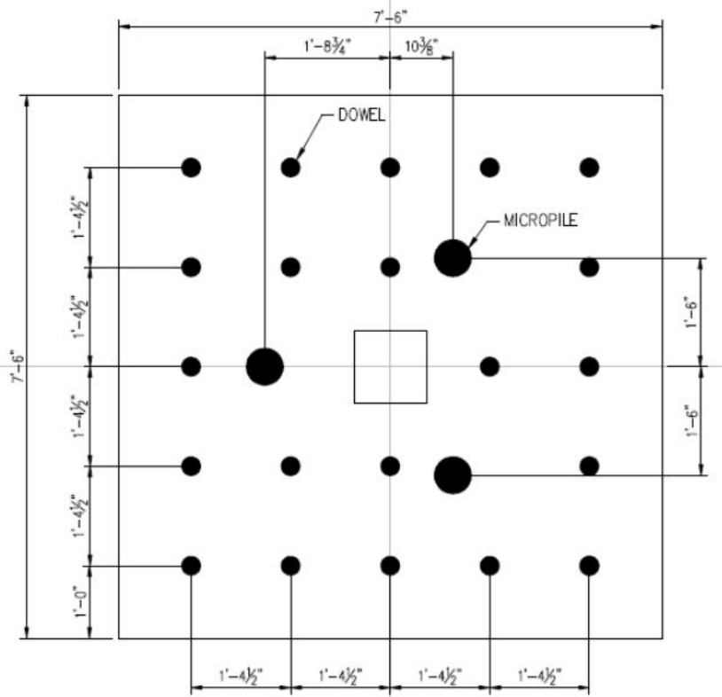
EXISTING FOOTING PLAN NO SCALE
