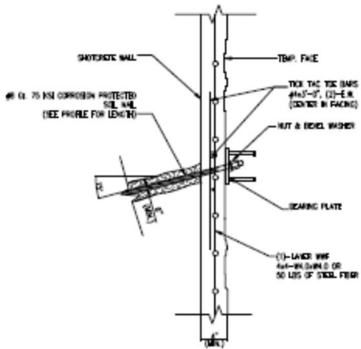
TEMPORARY SHOTCRETE FACE DETAIL NO SCALE
