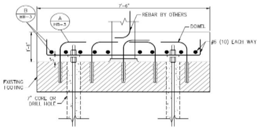
SECTION THROUGH EXISTING FOOTING NO SCALE
