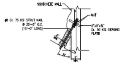
STRUT NAIL DETAIL NO SCALE
