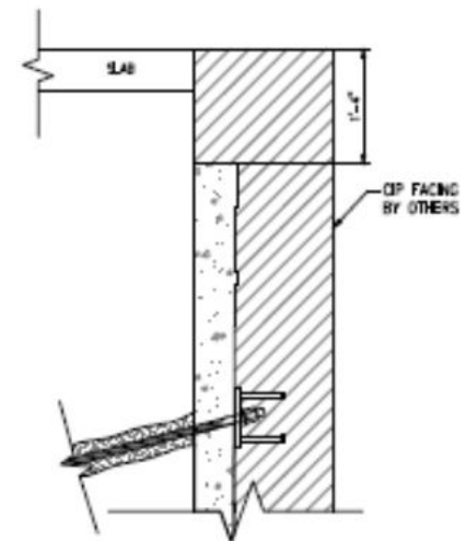
TOP OF WALL DETAIL NO SCALE
